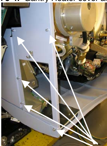
Illustration 3-4: Gantry Heater cover and filter holder Mounting Screws (new style cover shown)
