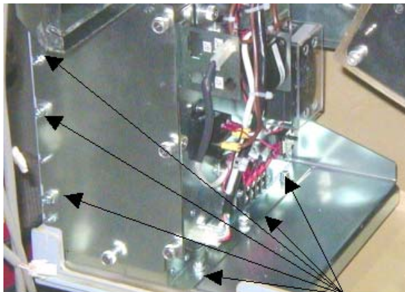
Illustration 2: Gantry Heater Mounting Screws
