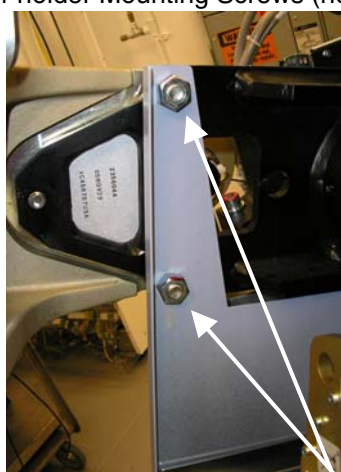
Illustration 3-4: Gantry Heater cover and filter holder Mounting Screws (new style cover shown)
