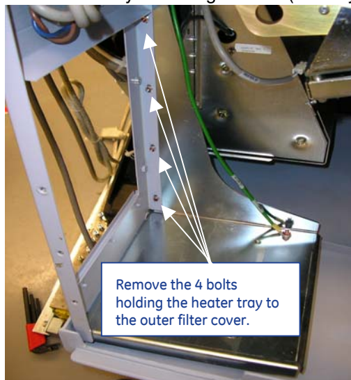
Illustration 5: Heater Tray Mounting Screws (new style cover shown)
