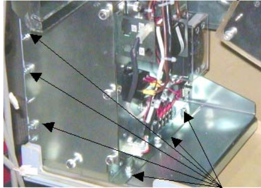
Illustration 7: Gantry Heater Mounting Screws
